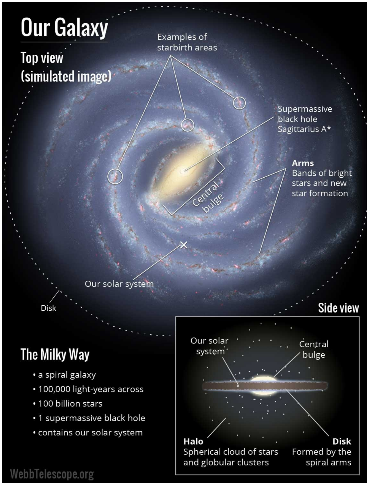
Our Galaxy Map (May 31, 2018)
